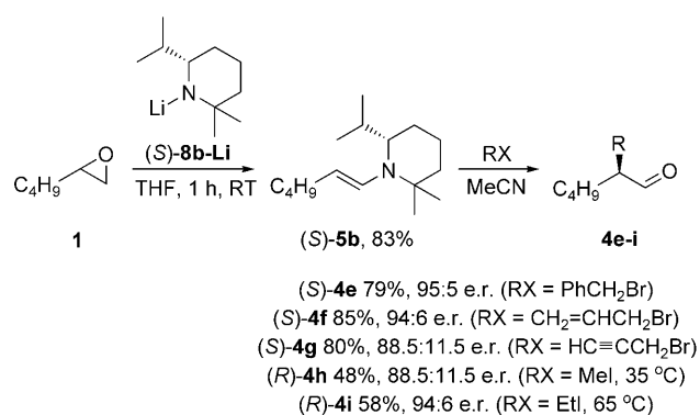
Scheme 4. Synthesis and asymmetric alkylation of enamine ( S )- 5b .
