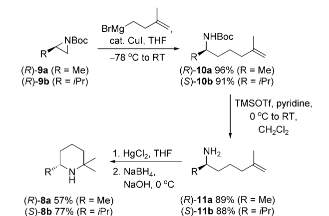
Scheme 2. Asymmetric synthesis of 6-alkyl-2,2-dimethylpiperidines ( R )- 8a and ( S )- 8b .
